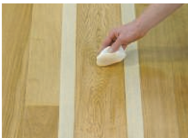
22) Thin application of Osmo Polyx®-Oil after leaving the first coat to dry thoroughly
